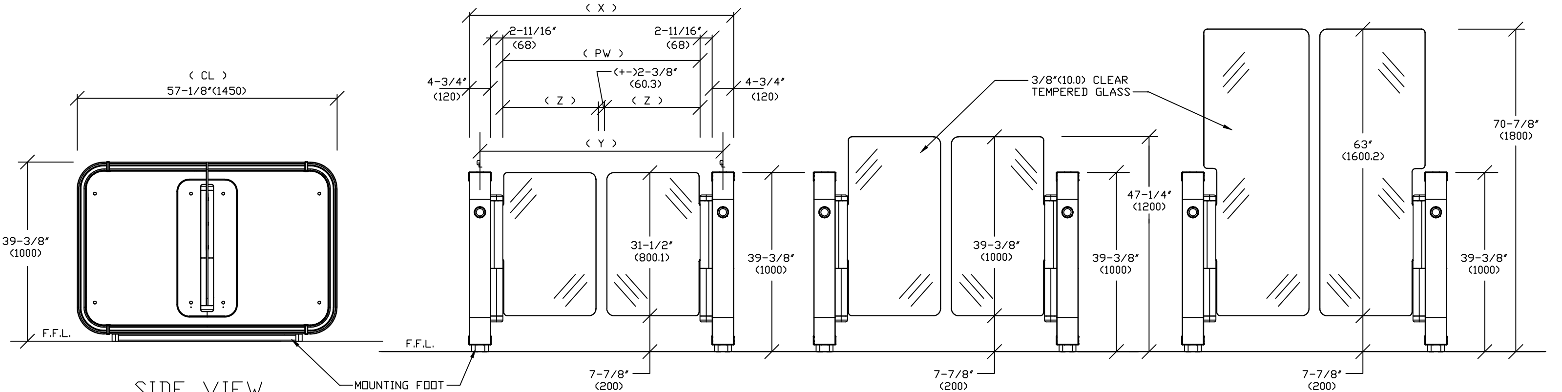
FRONT VIEW LOW GLASS
