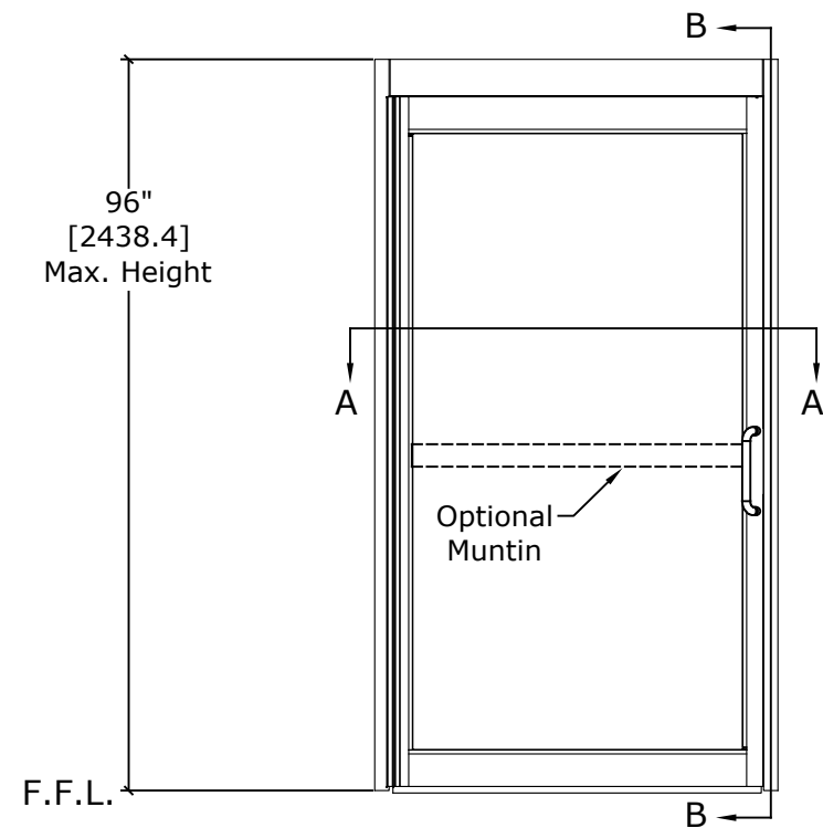
RH Single Panel Shown (LH Opposite)
