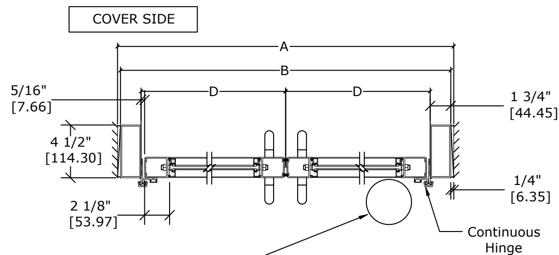
SECTION A-A SCALE - 1:8
