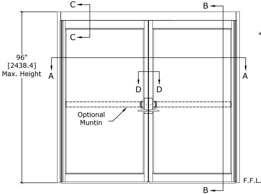
Equal Panel Shown SCALE - 1:25
