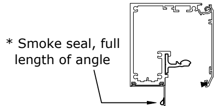
SECTION C-C SCALE - 1:5
