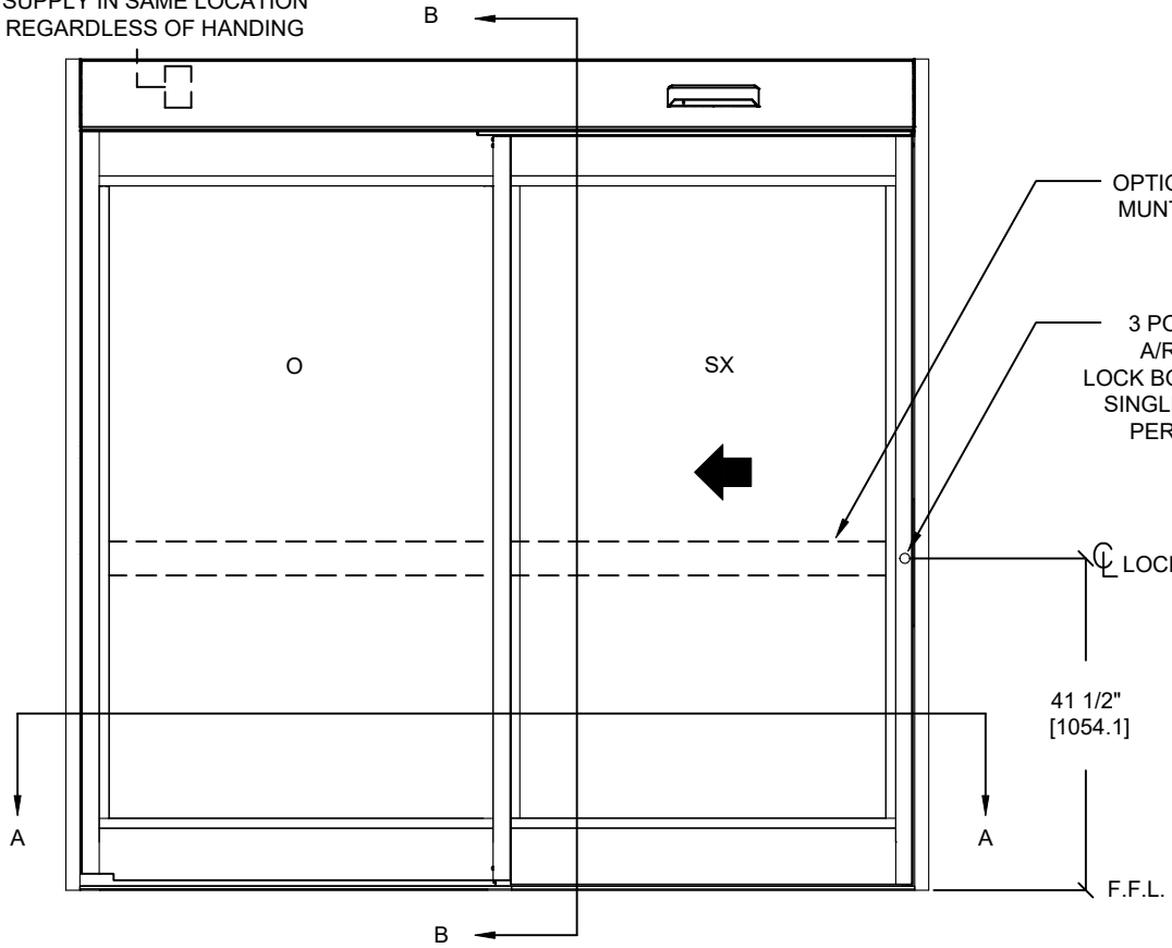
EXTERIOR ELEVATION
