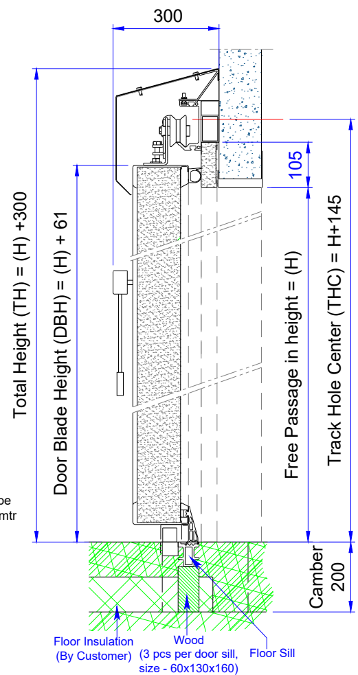
SECTION B-B
