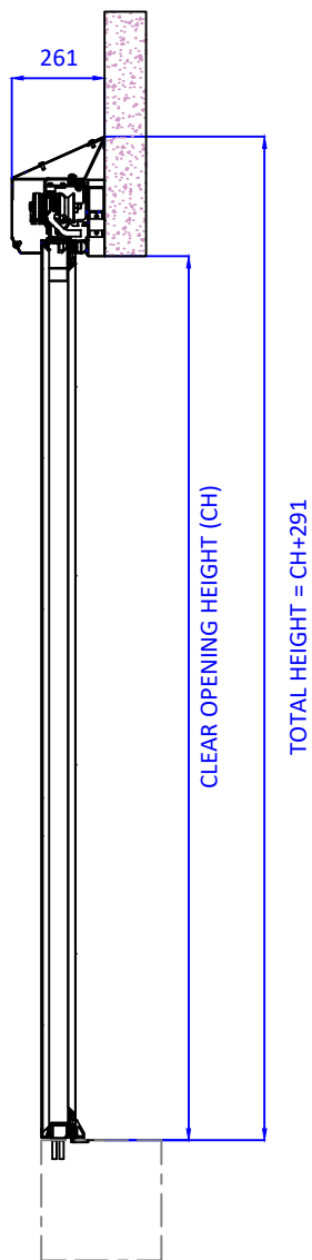
SECTION B-B
