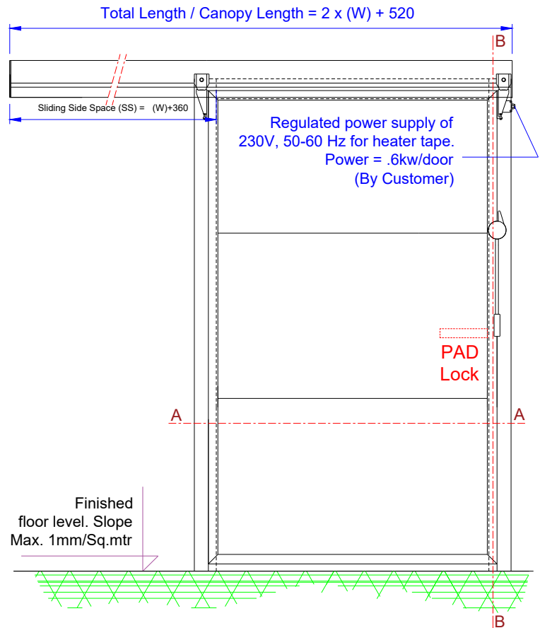
FRONT VIEW (Closed Position)
