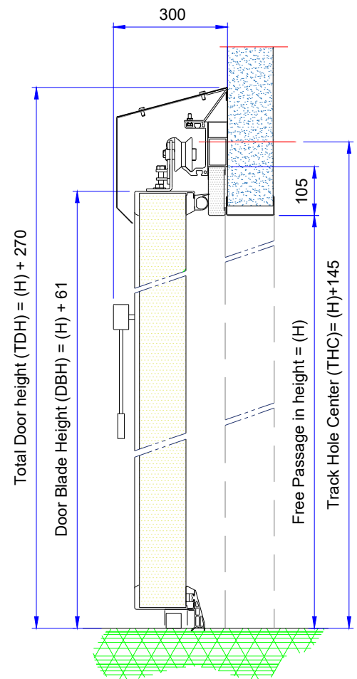
SIDE SECTIONAL VIEW
