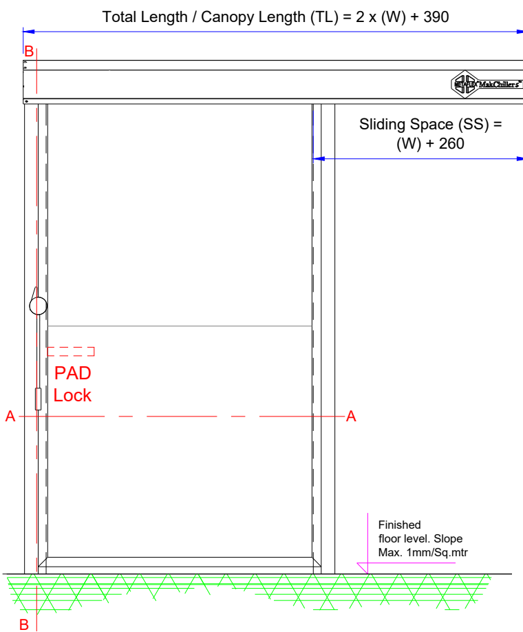
FRONT VIEW (Closed Position)
