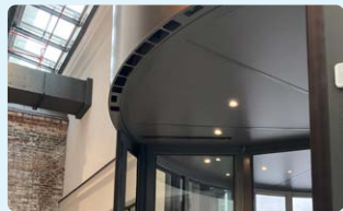
Horizontal air curtain with diffuser integrated in the canopy
