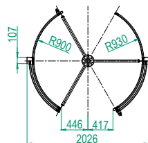
Top view open door
