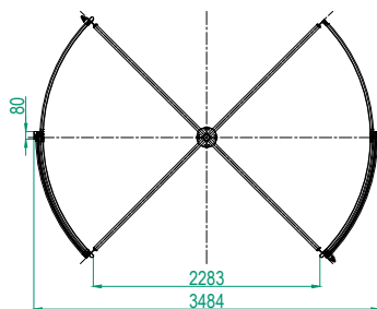
Top view open door
