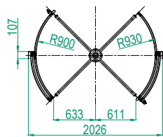
Top view open door
