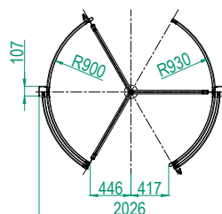
Top view open door
