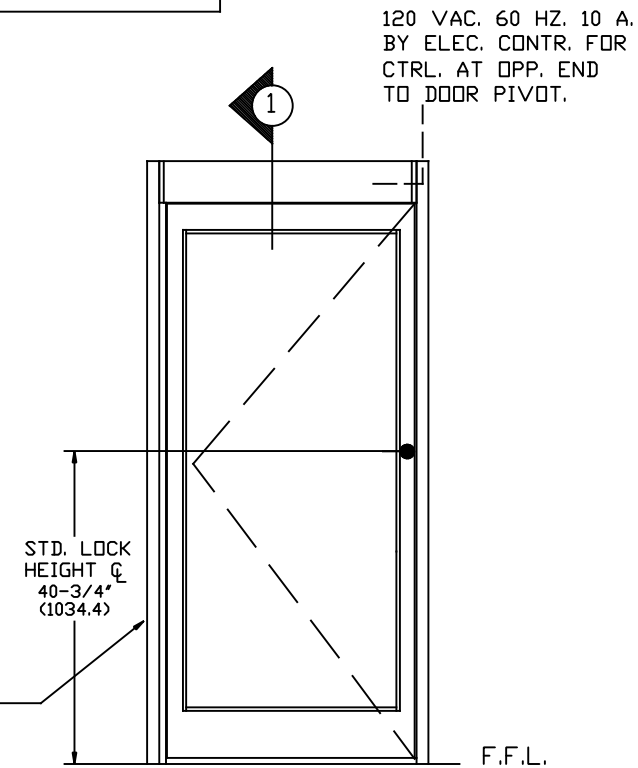
EXTERIOR ELEVATION (L.H. SHOWN/R.H. OPPOSITE) SW200i SERIES- SINGLE
