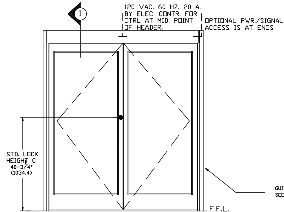
EXTERIOR ELEVATION SW200i SERIES- DUAL
