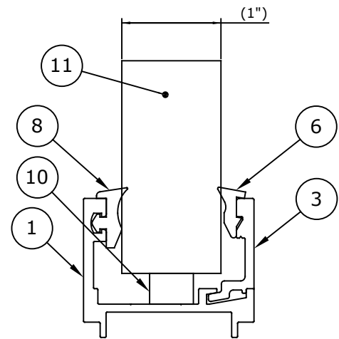
1" INSULATED IMPACT LEVEL D
