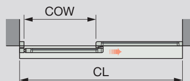
Right opening
