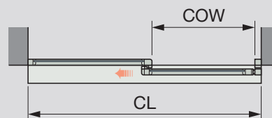
Left opening
